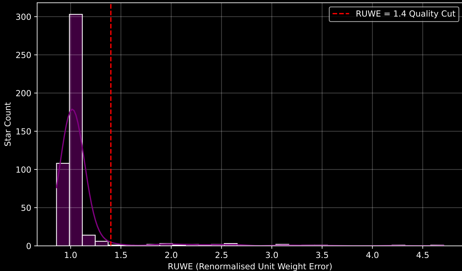
GAPOGEE DR17 Field [165-04] RUWE Distribution (n= 453)
