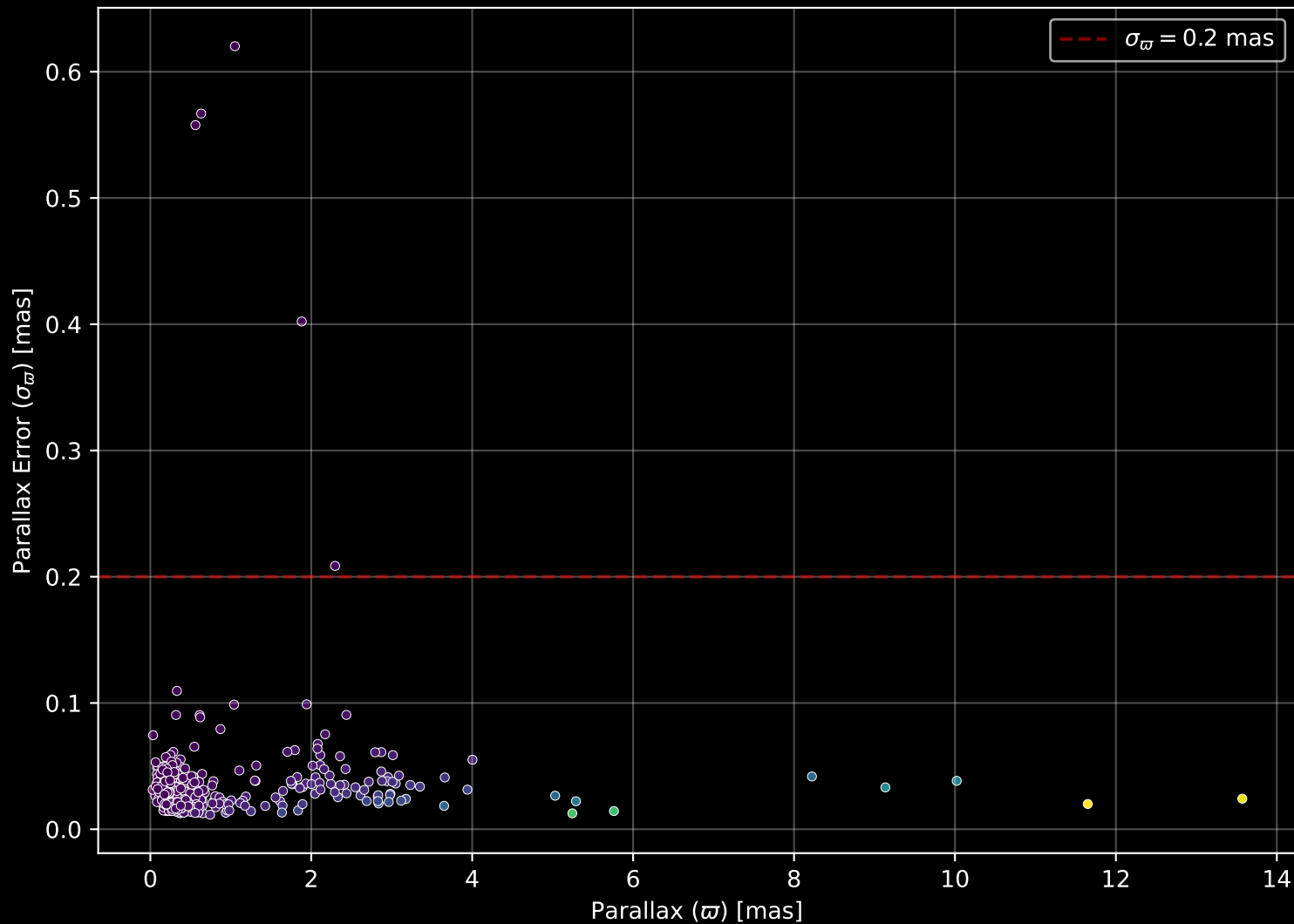
APOGEE DR17 Field: [165-04] Parallax Quality (n= 461)
