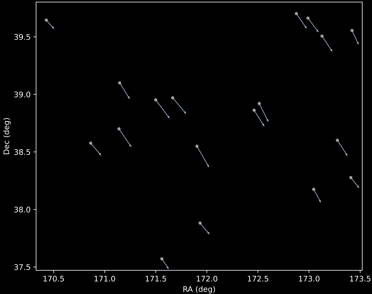
APOGEE DR17 Cluster 21 Proper Motion Vectors (n=18)
