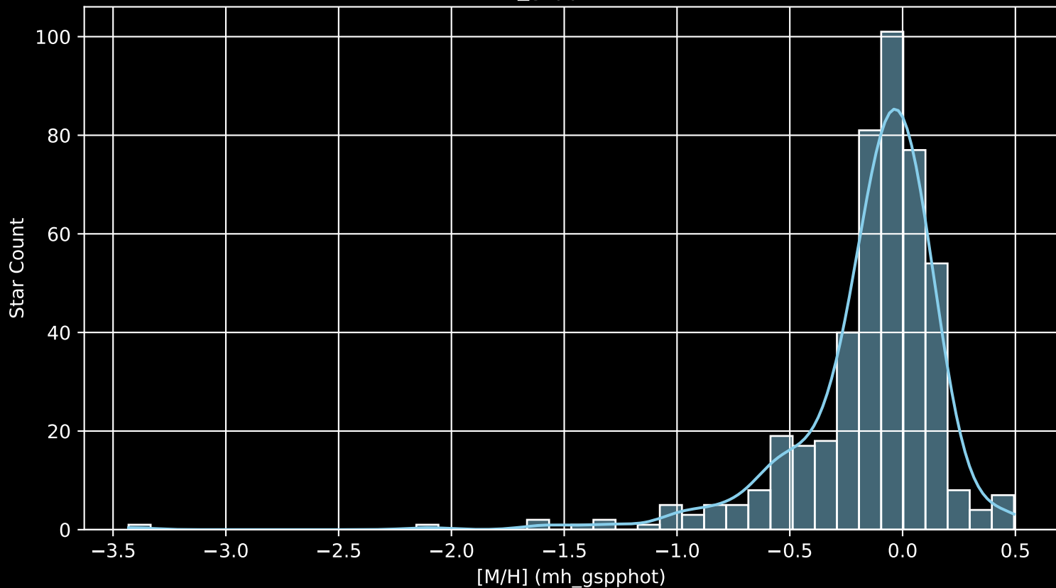
APOGEE DR17 Field: [165-04 [M/H] (mh_gspphot) (n= 460)
