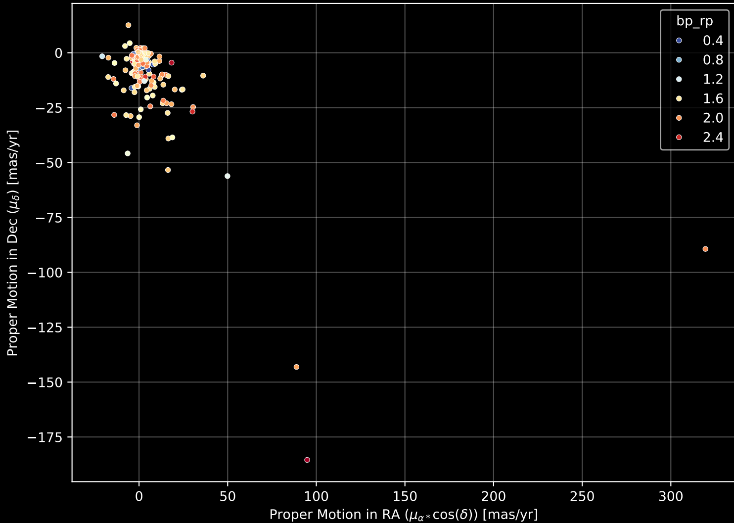
APOGEE DR17 Field: [165-04] Proper Motion Diagram (n= 461)
