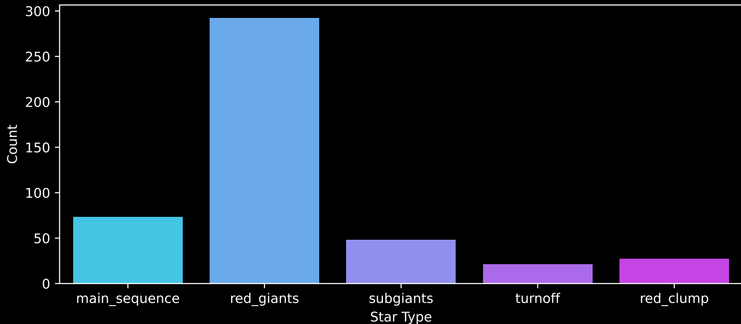
APOGEE DR17 Field: [165-04] Count plot of Star Type
