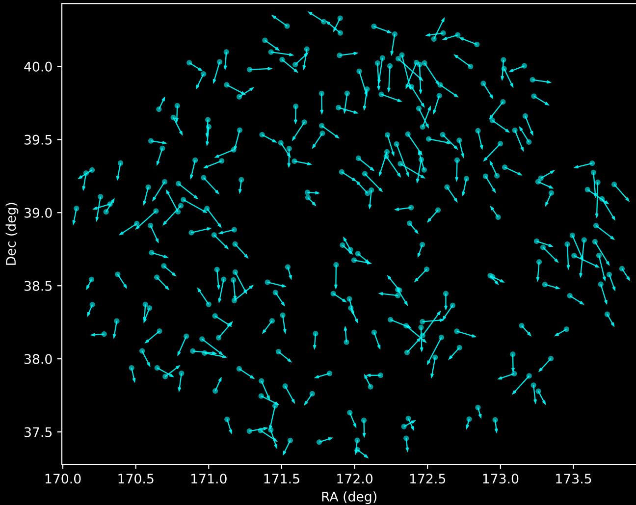
APOGEE DR17 Noise Stream Proper Motion Vectors (n=249)
