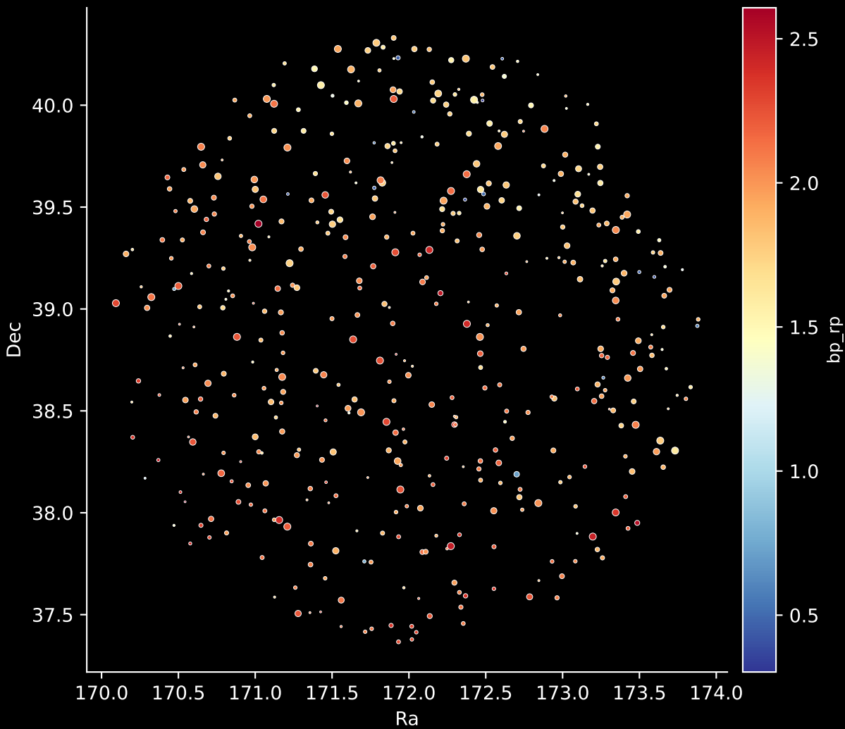
APOGEE DR17 Field: [165-04] Stars: 461
